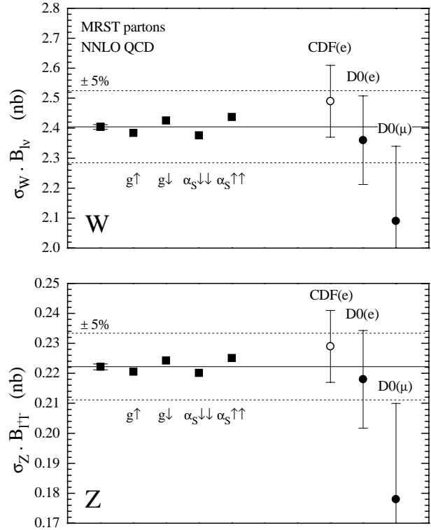
Fig. 38. Predictions for the W and Z production cross sections times leptonic branching ratios in p\bar{p} collisions at 1.8 TeV using the five MRST parton sets. The error bars on the default MRST prediction correspond to a scale variation of \mu = M_V/2 \rightarrow 2M_V , V = W, Z . Experimental measurements from CDF [60] and D0 [61] are shown
