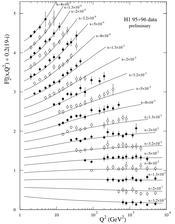
Fig. 7. Comparison of the F_2^p predictions of the MRST partons with the preliminary 1995 and 1996 nominal vertex data of H1 [27]. For display purposes we add 0.2(19-i) to F_2^p each time the value of x is decreased, where i = 1, 19 . These data are not used in the global analysis
