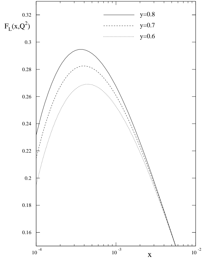
Fig. 17. Prediction for F_L at HERA versus x for y = 0.6, 0.7, 0.8 . Note that F_L has an implicit y dependence via the relation Q^2 = xys
