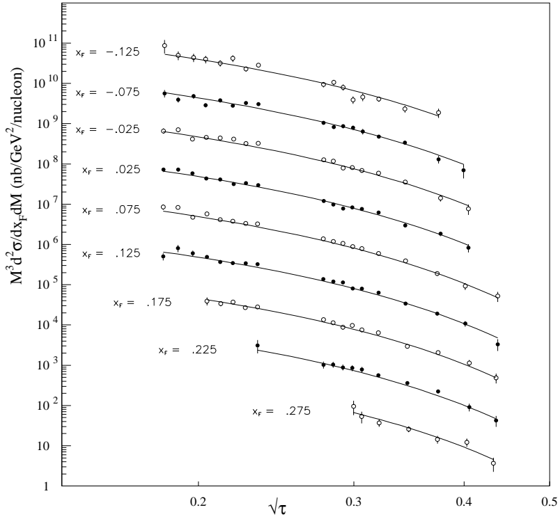
E772 (p d \rightarrow \mu^+ \mu^- X ) p_{LAB} = 800 GeV
