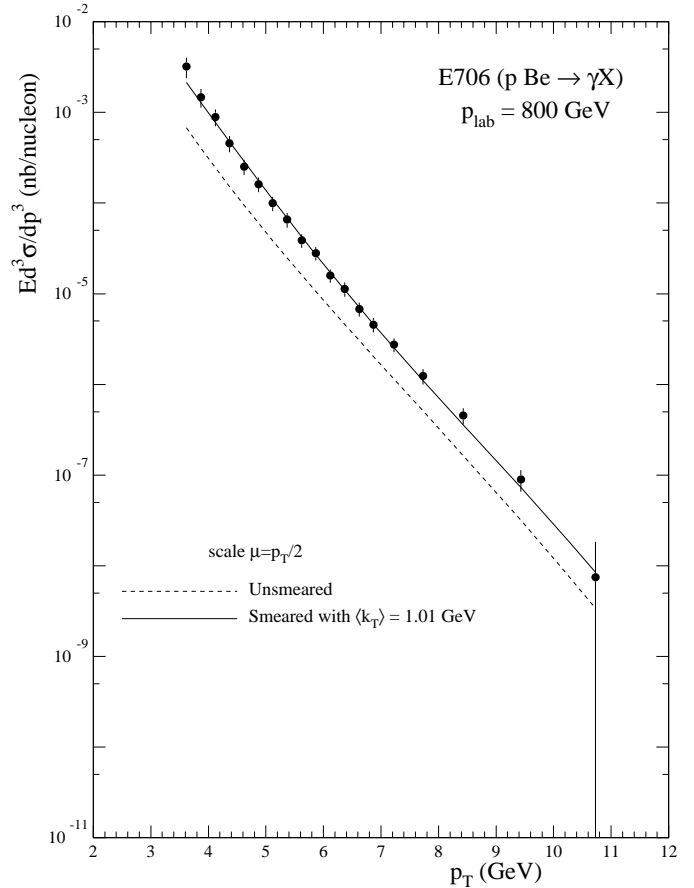
Fig. 25. Comparison of the E706 [8] data at 800 GeV with the MRST parton set. The scale is chosen to be p_T/2 and the effect of including parton transverse momentum is shown
