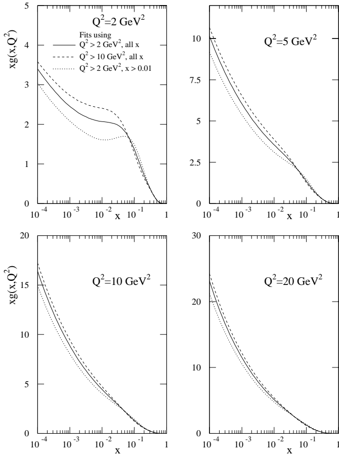
Fig. 19. The gluon distributions which result from making different cuts in Q^2 and x to the data included in the fits. The cuts which we use are specified in the first plot
