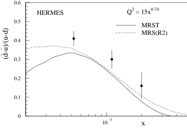
Fig. 33. Predictions for the ratio (\bar{d} - \bar{u})/(u - d) from the parton sets MRST and MRS(R2) compared with the preliminary estimates obtained by the HERMES collaboration [50] from their measurements of semi-inclusive pion production in DIS. Note that there is an additional overall systematic error on the data of \pm 0.07 . The Q^2 values of the data vary with x approximately according to the formula Q^2 (GeV ^2 ) = 15x^{0.74}
