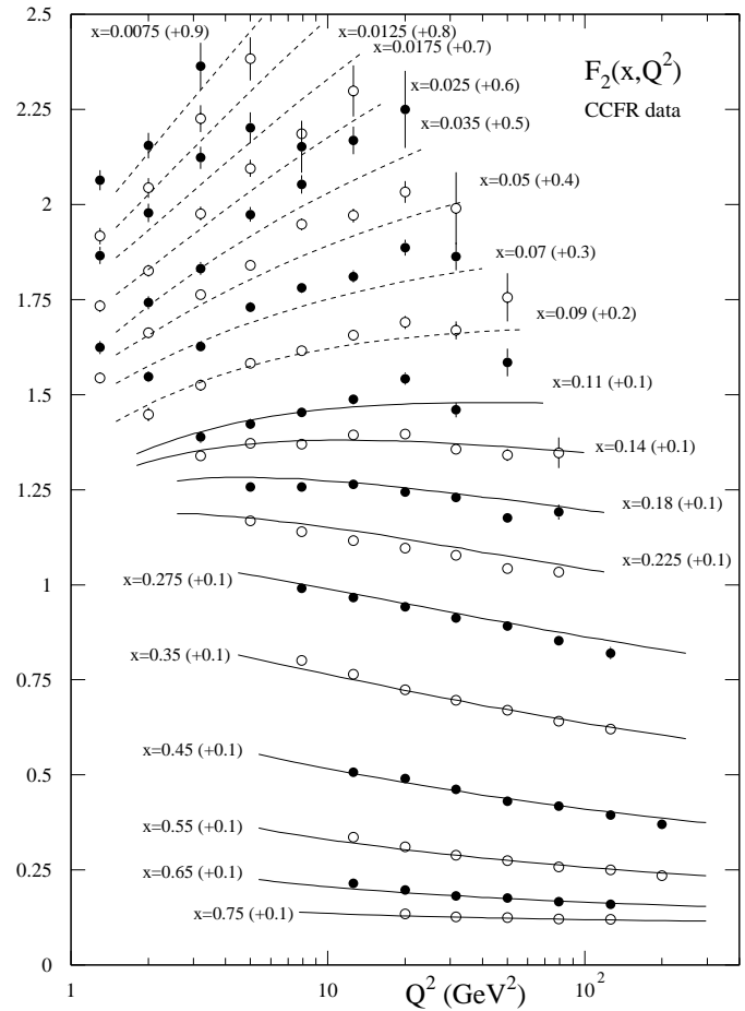
Fig. 11. The description of the CCFR [3] measurements of F_2^{pN} by the MRST partons. Only the data with x > 0.1 are included in the global fit. An x -dependent heavy target correction has been applied. The errors shown correspond to the quoted statistical errors together with a 1.5% uncertainty to represent the uncertainty of the heavy target correction. For display purposes we have added to F_2^{pN} the numbers shown in brackets
