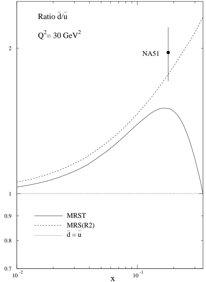
Fig. 32. The ratio of the parton distributions \bar{d}/\bar{u} at Q^2 = 30 \text{ GeV}^2 for the MRST and MRS(R2) parton sets compared to the estimate from the NA51 [11] measurement of the Drell-Yan asymmetry
