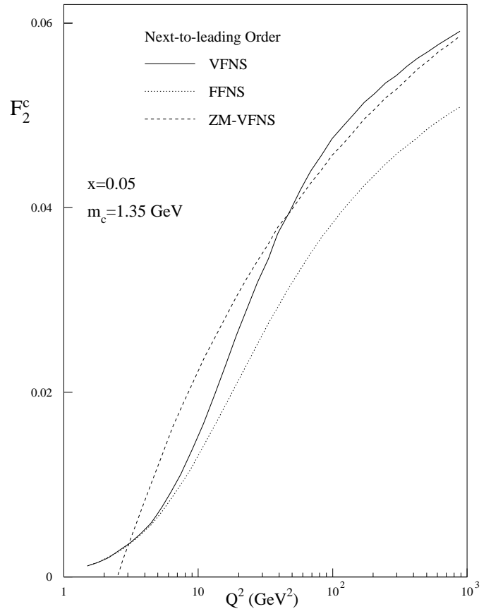
Fig. 26. The continuous curve is the MRST charm structure function at x = 0.05 obtained using the NLO prescription and NLO evolution (VFNS). For comparison, the prescriptions of the fixed flavour number scheme (FFNS) and the zero mass scheme (ZM-VFNS) are also shown
