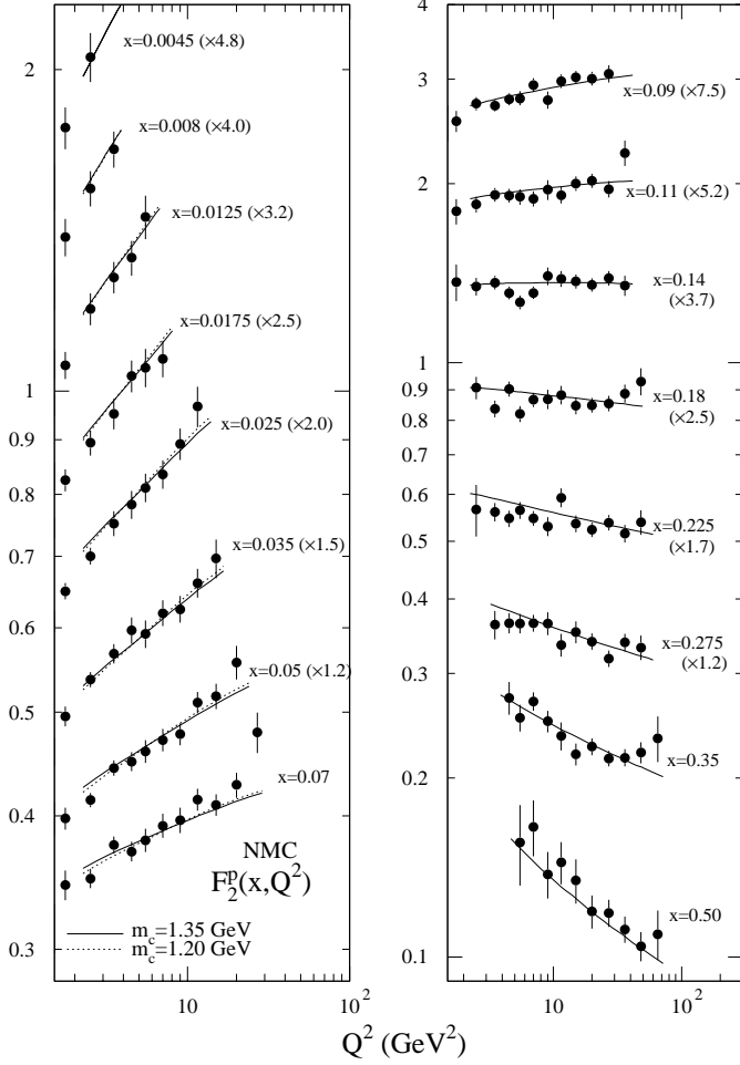
Fig. 8. Description of the NMC F_2^p data [13] by the MRST partons. The effect of lowering the charm quark mass from 1.35 to 1.20 GeV is shown by the dotted curve. For display purposes we have multiplied F_2^p by the numbers shown in brackets
