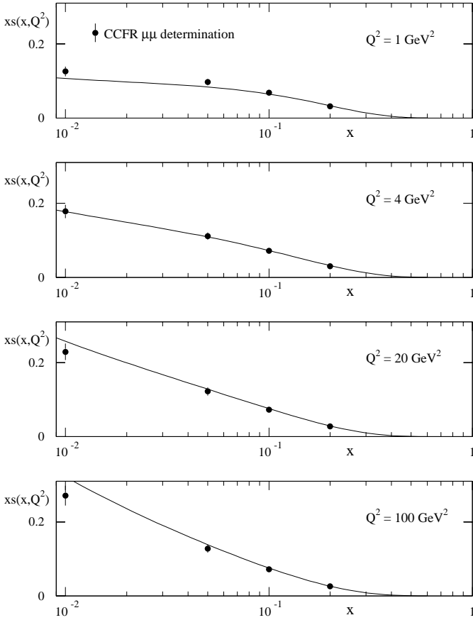
Fig. 30. Comparison of the strange quark distribution from the MRST set of partons compared with the determination of the strange sea obtained by the CCFR collaboration [16] in a NLO analysis of their data on the neutrino production of dimuons
