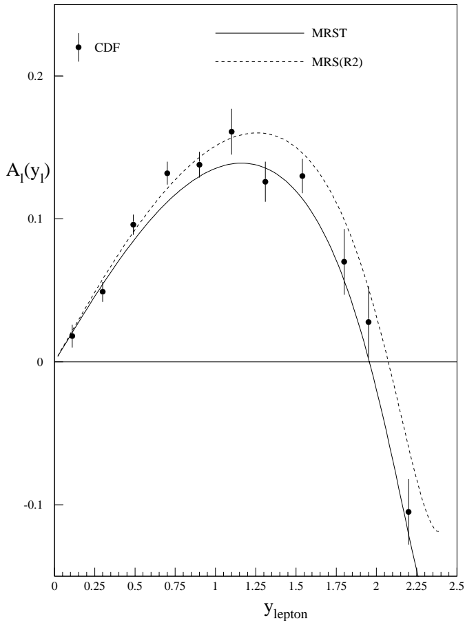
Fig. 35. The description of the lepton asymmetry for W^\pm production in p\bar{p} collisions at \sqrt{s} = 1.8 TeV. The data from CDF [12] are compared with the new MRST parton set and with the previous set MRS(R2)
