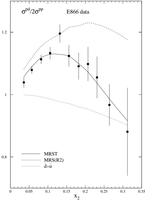
Fig. 31. The continuous curve is the MRST description of the E866 [10] data for the ratio of the cross sections for hadroproduction of dileptons for proton and deuterium targets versus x_2 , the fractional momentum of the parton in the target. The other curves are for comparison only
