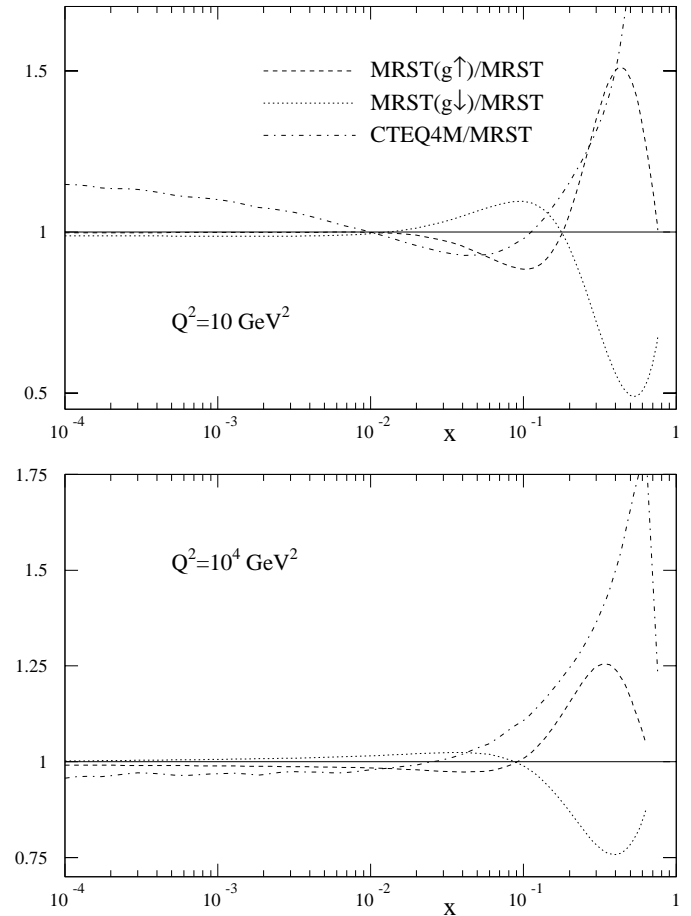
Fig. 2. The ratios of the g \uparrow and g \downarrow gluons to the ‘central’ gluon (MRST) at Q^2 = 10 and 10^4 GeV 2 . For comparison the ratio of the CTEQ4M [21] gluon to our central gluon is also shown
