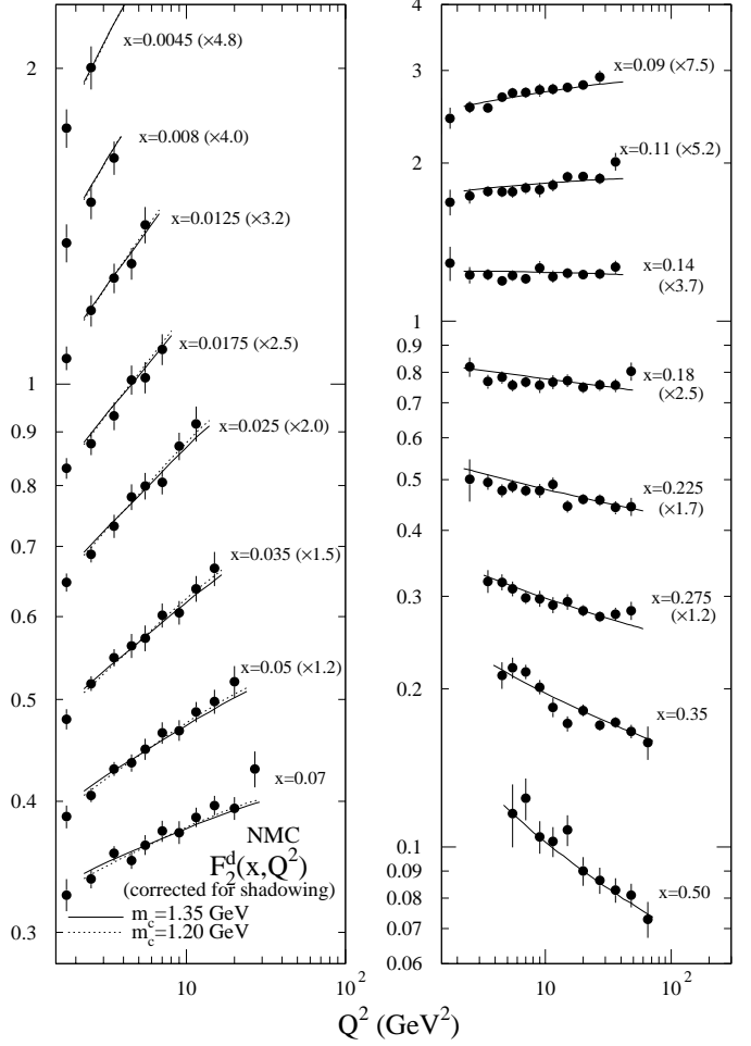
Fig. 9. Comparison of F_2^d from the MRST set with the NMC deuteron data [13]. The effect of lowering the charm quark mass from 1.35 to 1.20 GeV is shown. For display purposes we have multiplied F_2^d by the numbers shown in brackets
