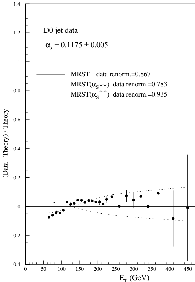
Fig. 43. As for Fig. 41 but including the comparisons with the \text{MRST}(\alpha_S \uparrow \uparrow) and \text{MRST}(\alpha_S \downarrow \downarrow) parton sets
