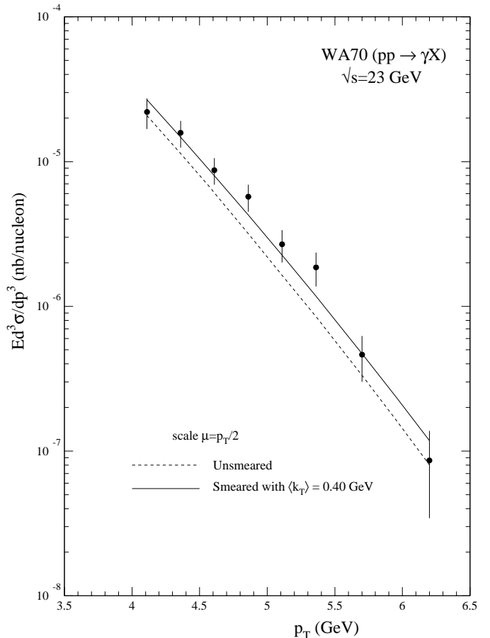
Fig. 23. Comparison of the WA70 [9] data with the MRST parton set with and without smearing in transverse momentum
