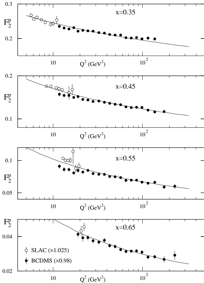
Fig. 10. The description of the large x BCDMS [23] and SLAC [25] measurements of F_2^p by the MRST partons
