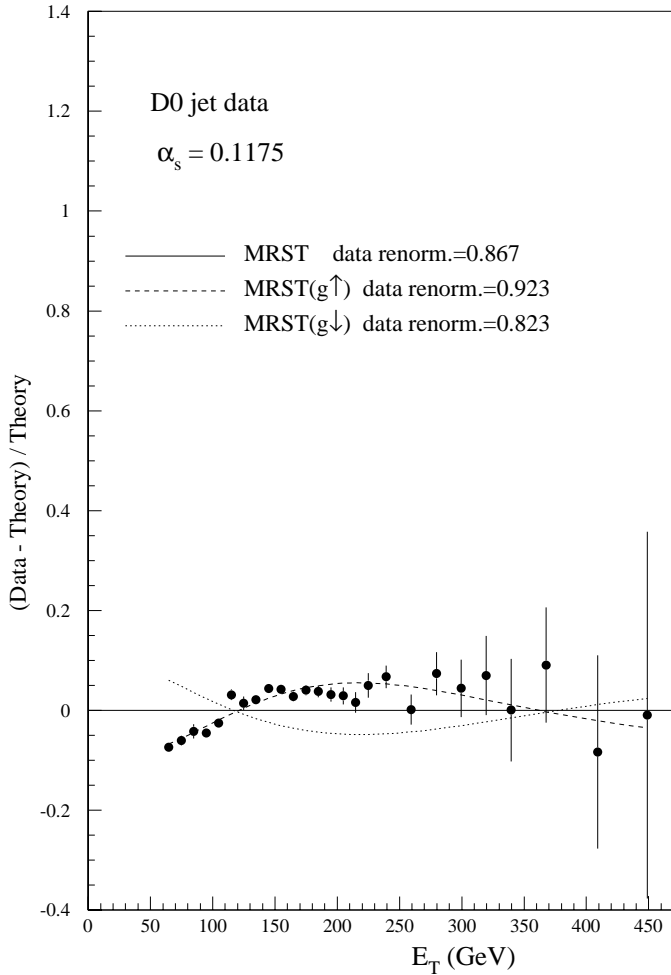
Fig. 41. The next-to-leading order QCD description of the D0 [38] single jet inclusive E_T distribution by the MRST set of partons. The overall normalization of the QCD prediction is fitted to the data. The comparisons with the MRST( g \uparrow ) and MRST( g \downarrow ) parton sets are also shown
