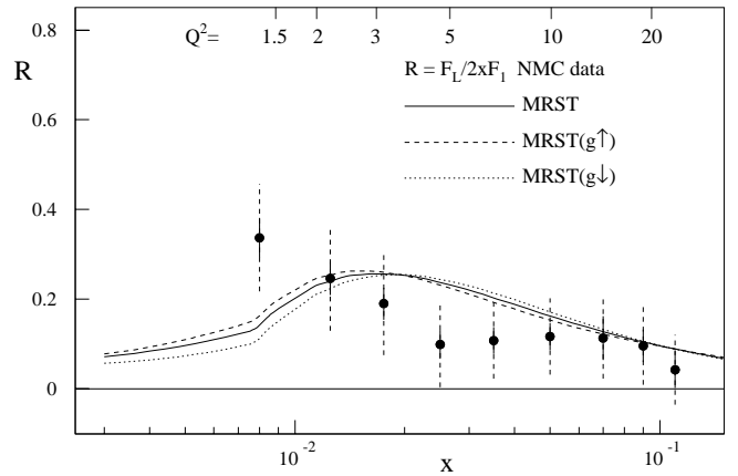
Fig. 18. Comparison of the predictions for R = F_L/2xF_1 with the NMC [13] data. The values of Q^2 appropriate to the data are given (in GeV 2 ) approximately by the formula Q^2 = 262x^{1.09} , and the corresponding scale is indicated on the upper edge of the plot
