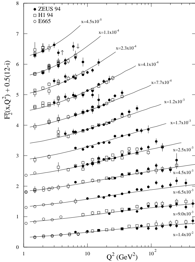
Fig. 6. The description of the F_2^p data at small x by the MRST set of partons. The comparison is made at twelve values of x chosen to be the most appropriate for the new HERA data. For display purposes we add 0.5(12-i) to F_2^p each time the value of x is decreased, where i = 1, 12 . The experimental data are assigned to the x value which is closest to the experimental x bin. Thus the ZEUS data [2] are shown in groupings with x values (3.5, 6.3, 6.5 \times 10^{-5}) , (1.02, 1.20 \times 10^{-4}) , (1.98, 2.53 \times 10^{-4}) , (4.0, 4.5 \times 10^{-4}) , (6.32, 8.00 \times 10^{-4}) , (1.02, 1.20 \times 10^{-3}) , (1.612 \times 10^{-3}) , (2.53, 2.60 \times 10^{-3}) , (4.00 \times 10^{-3}) , (6.325 \times 10^{-3}) , (1.02 \times 10^{-2}) , (1.612 \times 10^{-2}) , and the H1 data [1] in groupings with x values (3.2, 5.0 \times 10^{-5}) , (0.80, 1.30 \times 10^{-4}) , (2.0, 2.5 \times 10^{-4}) , (3.2, 5.0 \times 10^{-4}) , (6.3, 8.0 \times 10^{-4}) , (1.3 \times 10^{-3}) , (1.585 \times 10^{-3}) , (2.0, 2.5, 3.2 \times 10^{-3}) , (3.98, 4.0, 5.0 \times 10^{-3}) , (6.3 \times 10^{-3}) , (8.0 \times 10^{-3}) , (1.3 \times 10^{-2}) . The E665 data [24], which are shown on the curves with the five largest x values, are measured at x = (2.46 \times 10^{-3}) , (3.698, 5.2 \times 10^{-3}) , (6.934 \times 10^{-3}) , (8.933 \times 10^{-3}) , (1.225, 1.73 \times 10^{-2}) .
