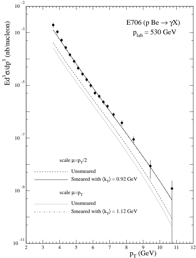
Fig. 24. Comparison of the E706 [8] data at 530 GeV with the MRST parton set. The results for two choices of the factorization scale are shown, together with the improvement of the description obtained by including parton transverse momentum in each case. The two ‘improved’ curves lie on top of each other
