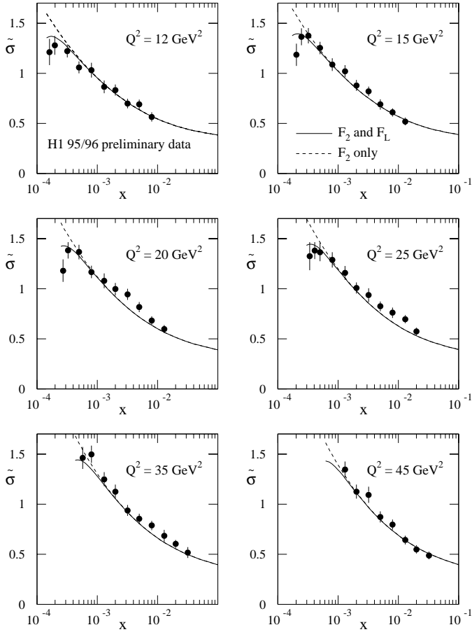
Fig. 16. The description of the quantity \tilde{\sigma} = F_2 - y^2/[1 + (1-y)^2]F_L compared with the preliminary H1 1995/96 [27] data. Also shown (dashed curve) is the contribution to \tilde{\sigma} of F_2 only
