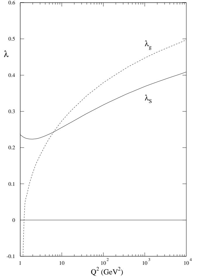
Fig. 13. The effective exponents \lambda_S, \lambda_g of the small x behaviour of the sea-quark and gluon distributions of the default MRST partons versus Q^2 , defined such that xS \sim x^{-\lambda_S} and xg \sim x^{-\lambda_g}
