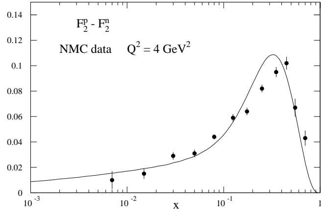
Fig. 34. The MRST description of the difference F_2^p - F_2^n at Q^2 = 4 GeV ^2 compared with the measurements from NMC [51]
