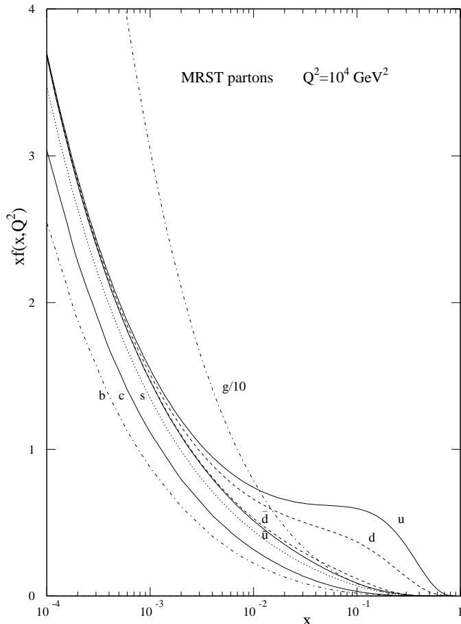
Fig. 4. MRST partons at Q^2 = 10^4 \text{ GeV}^2
