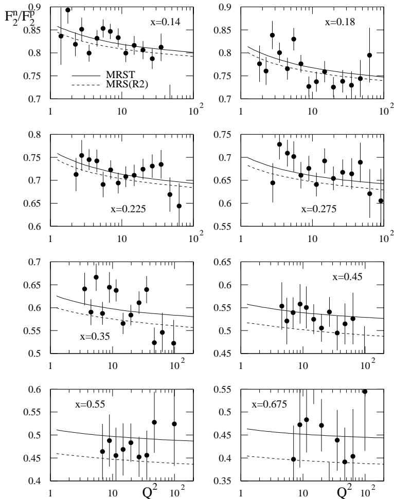
Fig. 36. The large x data on the ratio F_2^n/F_2^p extracted from the measurements of F_2^d/F_2^p by NMC [13] compared with the MRST and MRS(R2) descriptions
