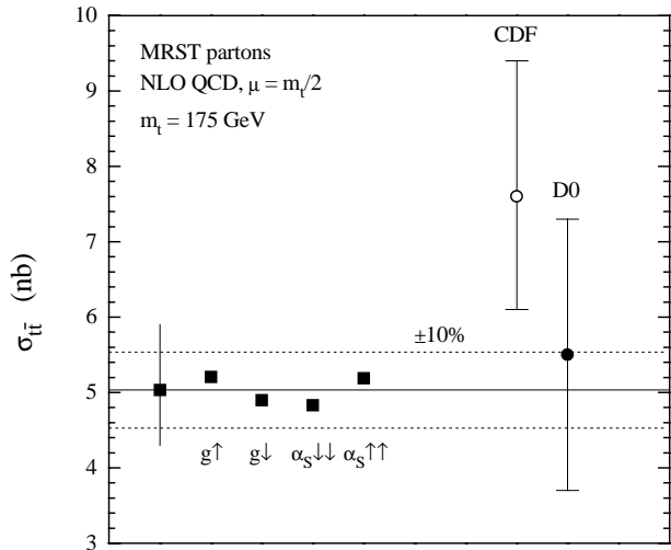
Fig. 39. Predictions for the t\bar{t} total cross section in p\bar{p} collisions at 1.8 TeV using the five MRST parton sets. The error bars on the default MRST prediction correspond to a variation in the top mass of \pm 5 GeV. Experimental measurements from CDF [65] and D0 [66] are shown
