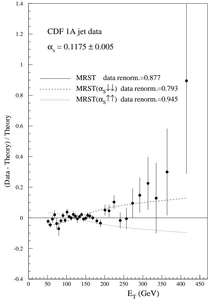
Fig. 42. As for Fig. 40 but including the comparisons with the MRST( \alpha_S \uparrow \uparrow ) and MRST( \alpha_S \downarrow \downarrow ) parton sets
