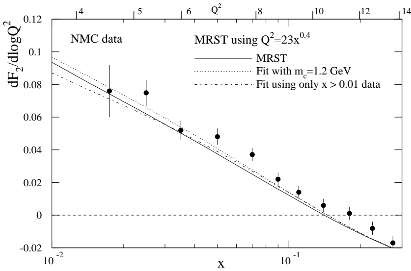
Fig. 15. The continuous curve is the description of the slopes \partial F_2/\partial \ln Q^2 of the NMC proton data. The experimental points were computed from linear fits to the data in Fig. 8. We also show the effect of modifying the charm quark mass and of excluding low x data (with x < 0.01 ) from the global fit
