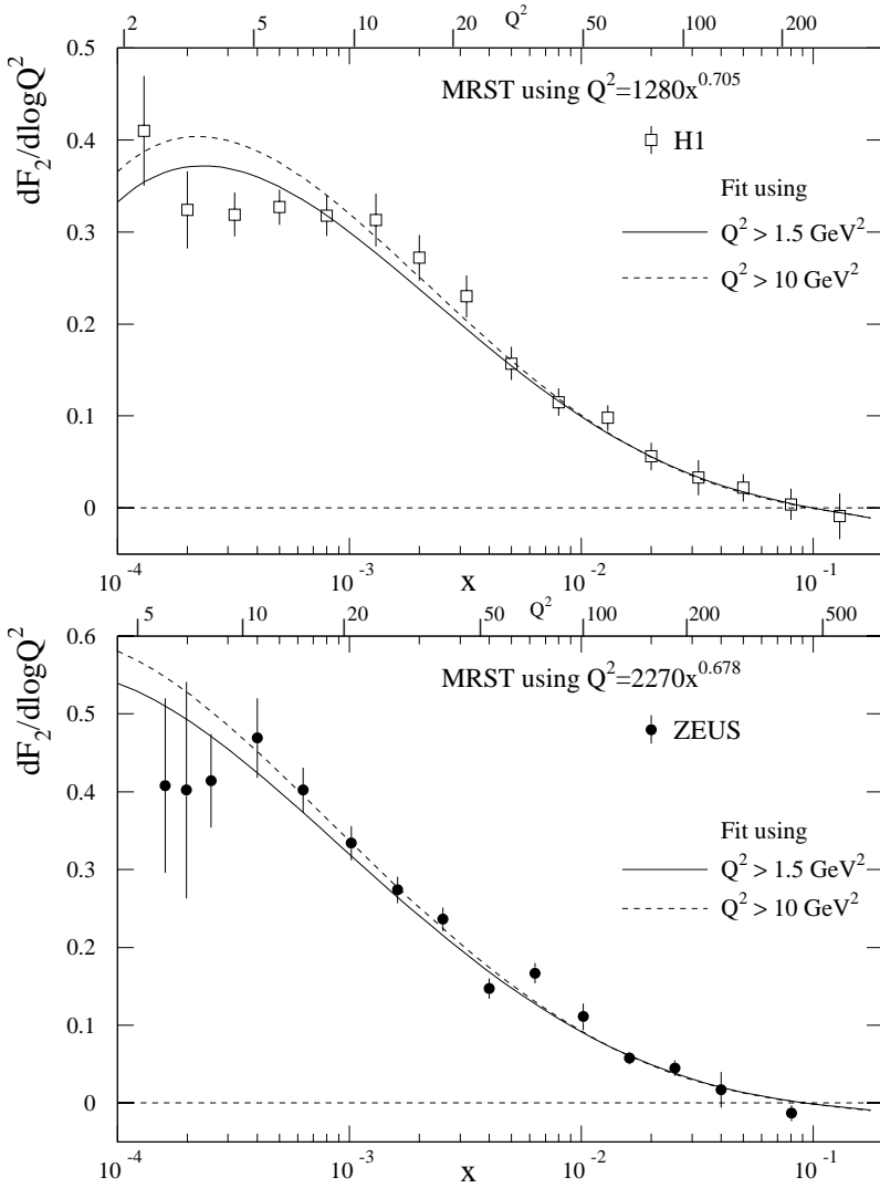
Fig. 14. The description of the slopes \partial F_2/\partial \ln Q^2 versus x for the HERA data. The experimental points were computed from linear fits to the data in Fig. 6. The solid curve corresponds to the MRST set while the dashed line indicates the effect of removing low Q^2 data (with Q^2 < 10 \text{ GeV}^2 ) from the fit. The values of Q^2 appropriate to the data are given (in \text{GeV}^2 ) approximately by the formulae shown and the corresponding scale is indicated on the upper edge of each plot
