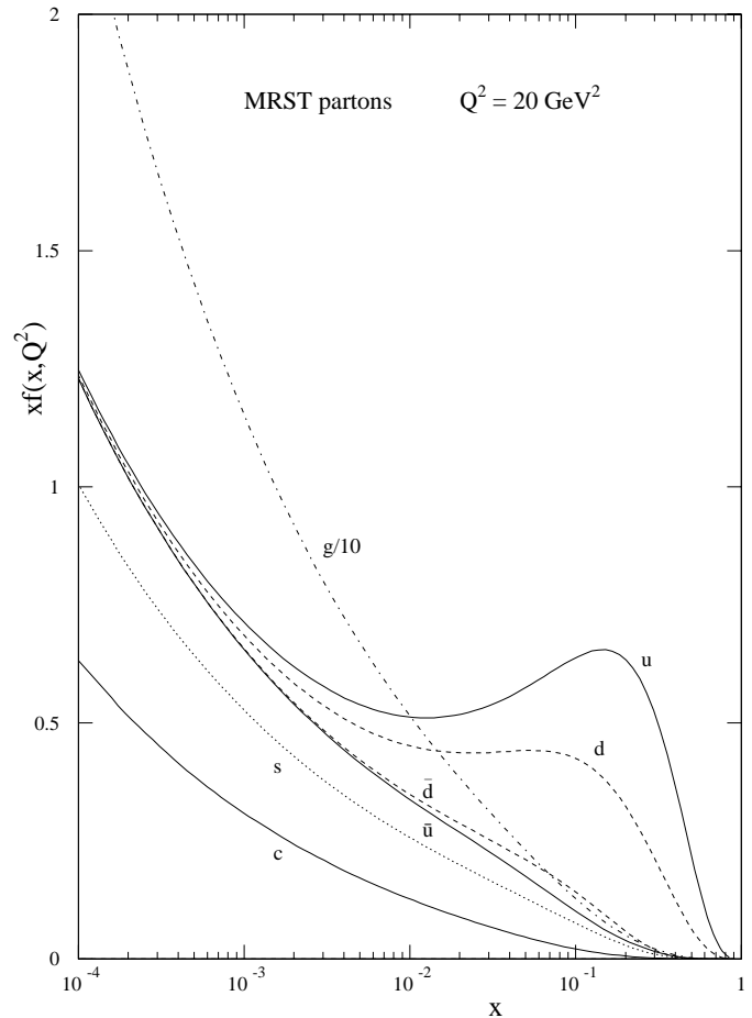
Fig. 3. MRST partons at Q^2 = 20 \text{ GeV}^2
