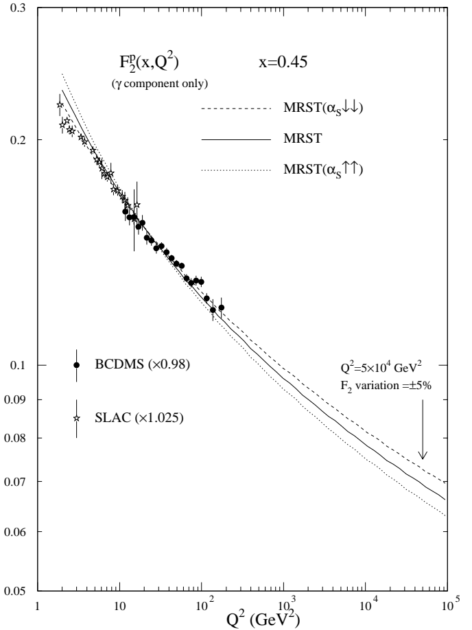
Fig. 22. The extrapolation of the fits at x = 0.45 to high Q^2 using the MRST, MRST( \alpha_S \uparrow\uparrow ) and MRST( \alpha_S \downarrow\downarrow ) set of partons
