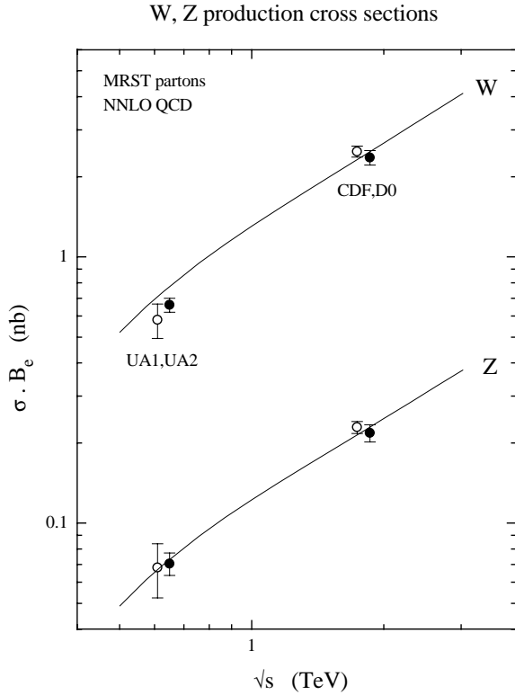
Fig. 37. Total W, Z production cross sections times leptonic branching ratios as a function of the (p\bar{p}) collider energy \sqrt{s} , calculated using the default MRST partons. Experimental measurements from UA1 [58], UA2 [59], CDF [60] and D0 [61] are also shown
