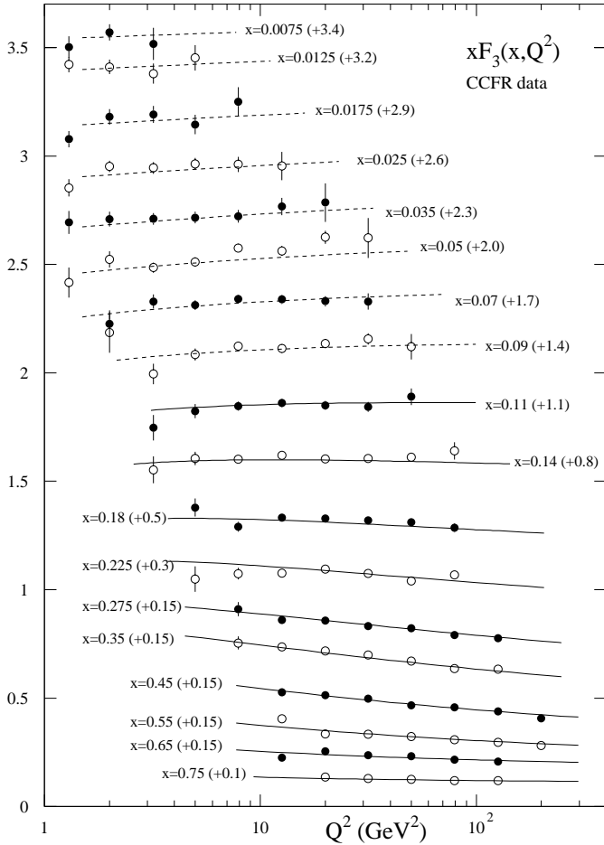
Fig. 12. The same as Fig. 11 but for the structure function xF_3^{vN}
