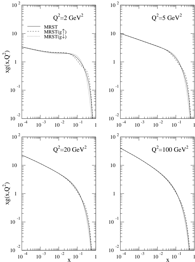
Fig. 1. The gluon distributions at Q^2 = 2, 5, 20 and 100 \text{ GeV}^2 corresponding to the MRST, MRST( g \uparrow ) and MRST( g \downarrow ) sets of partons with, respectively, the central, larger and smaller gluon at large x . We take MRST as the default set of partons throughout the paper
