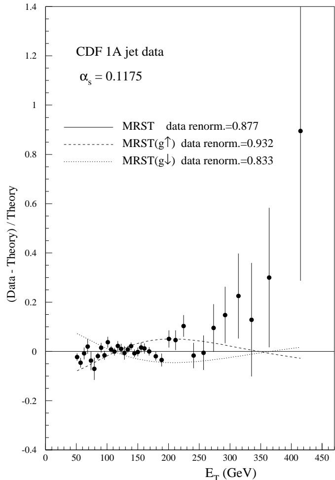
Fig. 40. The next-to-leading order QCD description of the CDF [37] single jet inclusive E_T distribution by the MRST set of partons. The overall normalization of the QCD prediction is fitted to the data. The comparisons with the MRST( g \uparrow ) and MRST( g \downarrow ) parton sets are also shown
