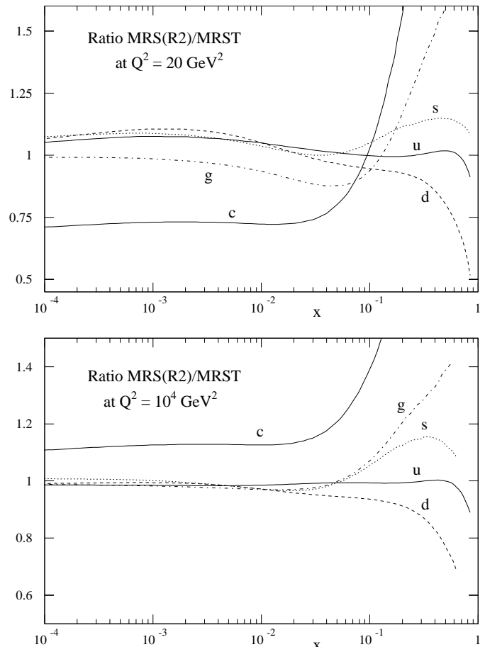
Fig. 5. Comparison of the MRST partons with those of the previous MRS(R2) set at Q^2 = 20 \text{ GeV}^2 (upper plot) and Q^2 = 10^4 \text{ GeV}^2 (lower plot)
