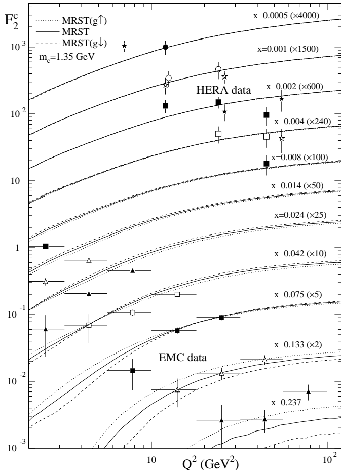
Fig. 27. The prediction for the charm structure function using the three MRST parton sets characterized by the different large x gluon behaviour. The HERA data at small x are from H1 [5] and ZEUS [6], and the large x data are from EMC [7]
